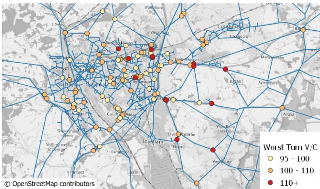
Figure 21 - Worst Turn V/C AM
