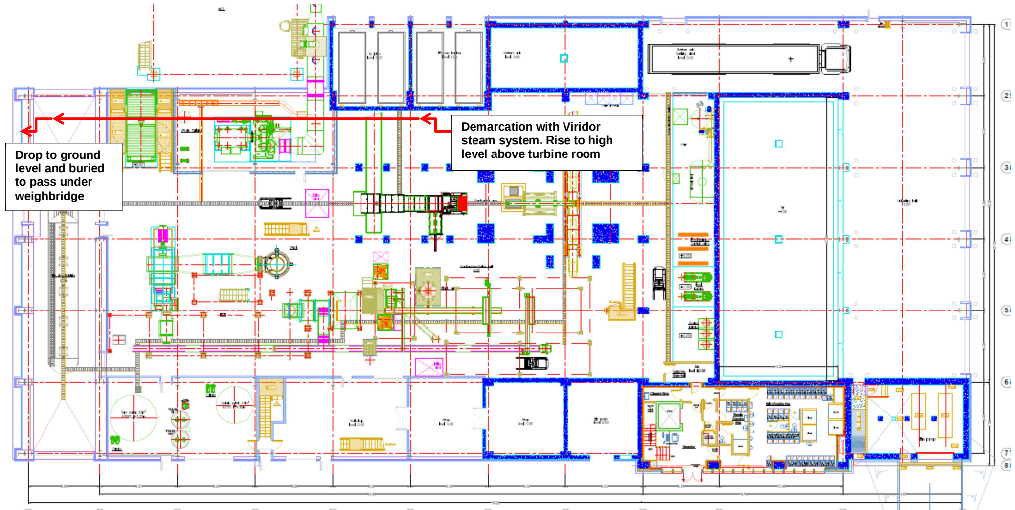
Figure 4-6: Steam pipe route inside EfW
