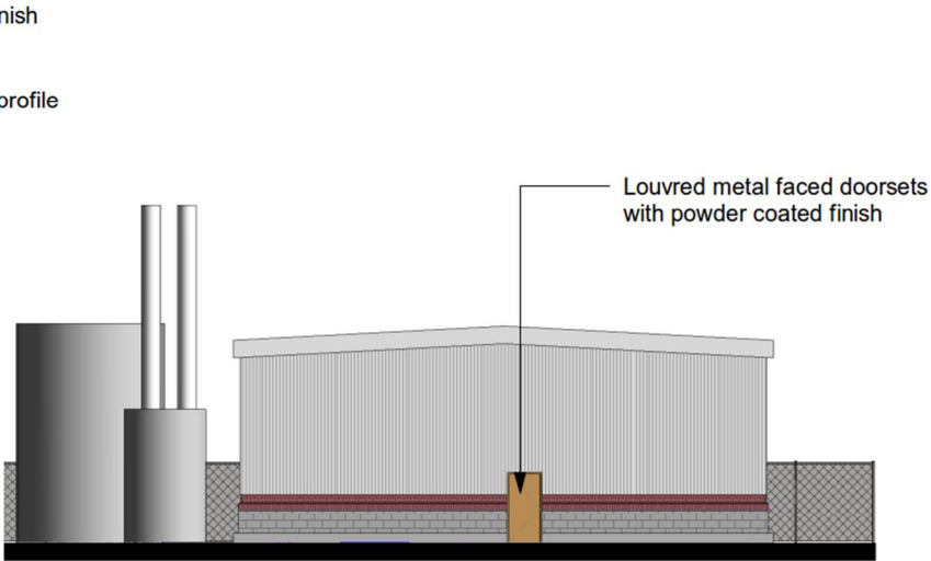
NW Elevation 1 : 200
