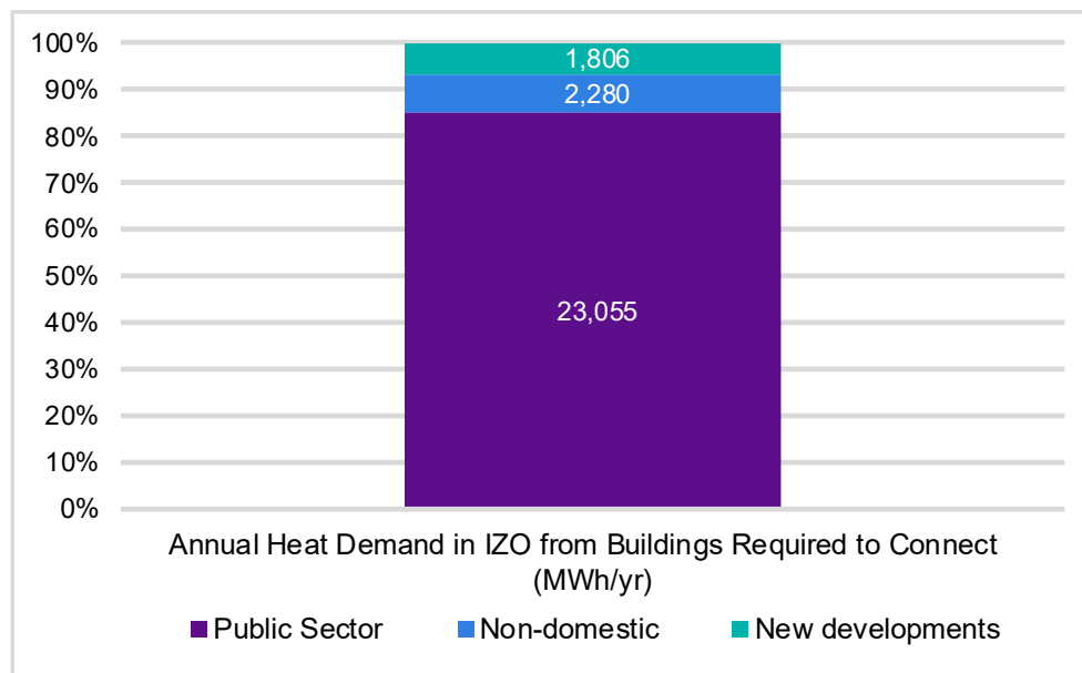
Figure 15: Exeter University Streatham - Categorisation of Heat Demand for Buildings Potentially Required to Connect in the IZO
